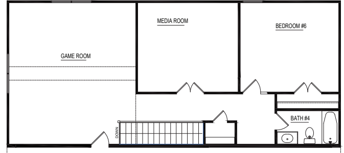
OPTIONAL THIRD FLOOR
