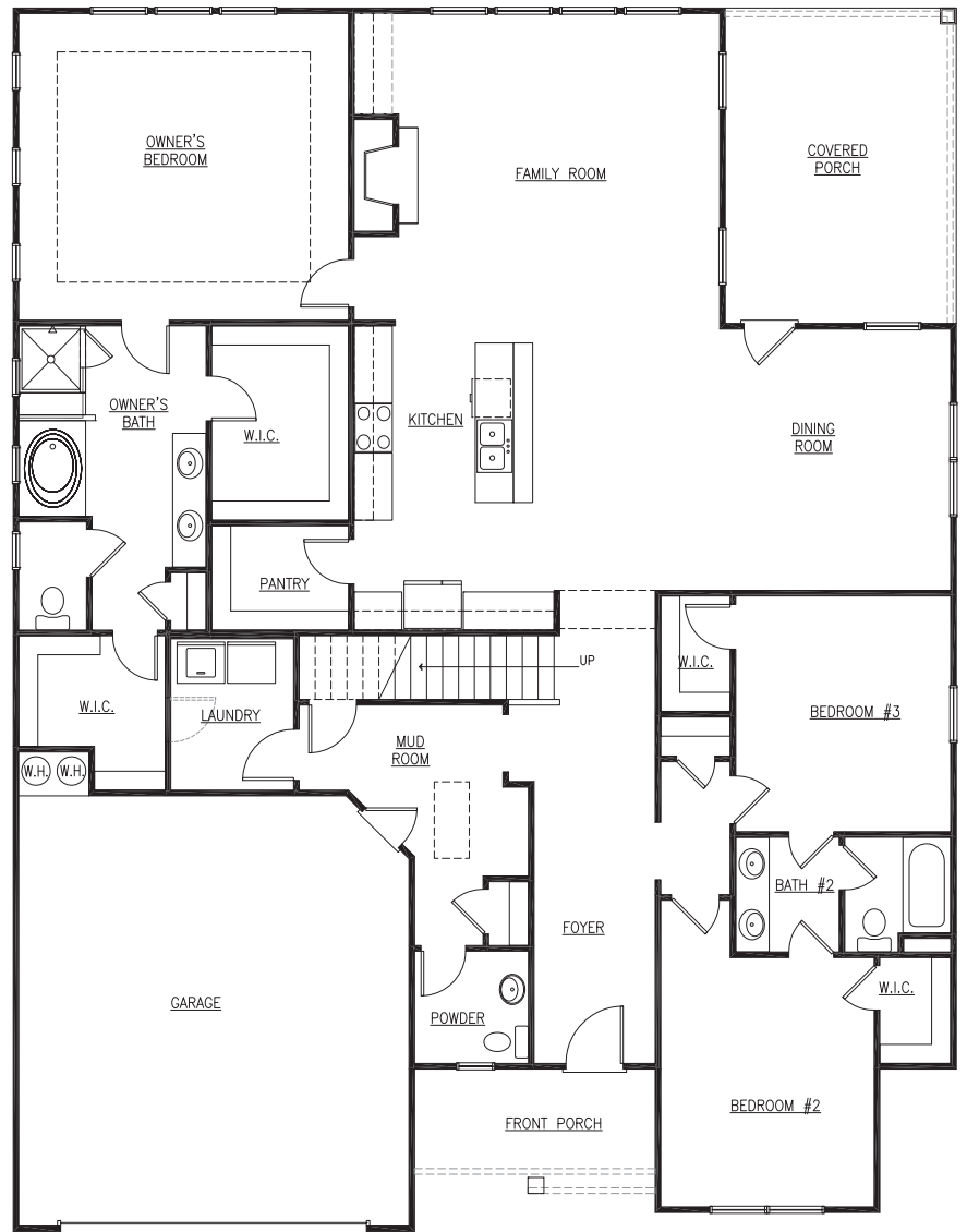
FIRST FLOOR
