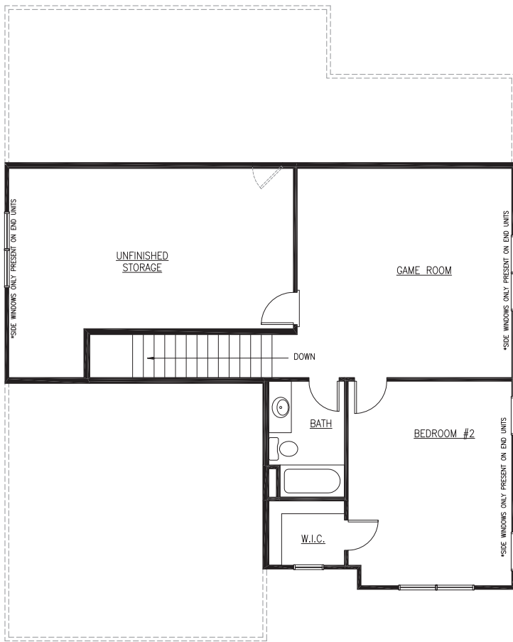
SECOND FLOOR
